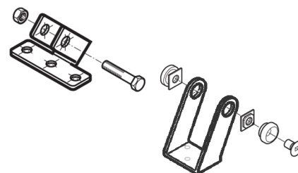
Kit actuator support bracket
